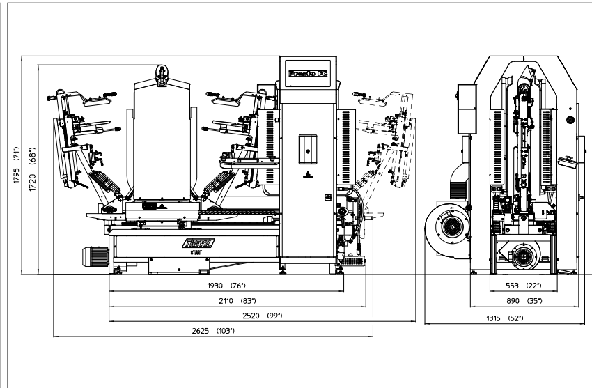
Figure 2.2 - Machine dimensions
